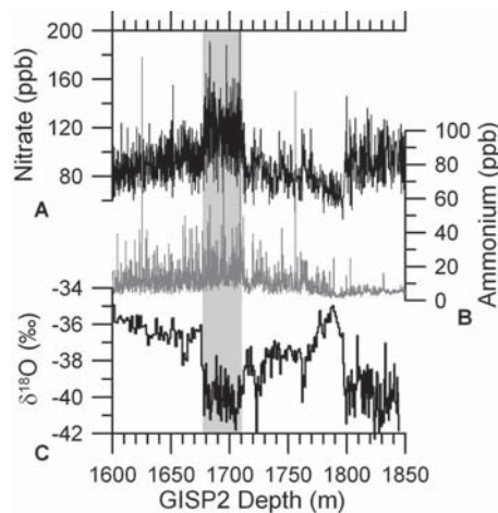
Figure 1. Nitrate (A), ammonium (B), and \delta^{18}\text{O} (C) records from Greenland Ice Sheet Project 2 (GISP2) (Grootes et al., 1993; Mayewski et al., 1997). Gray bar denotes the Younger Dryas Cold Event.
