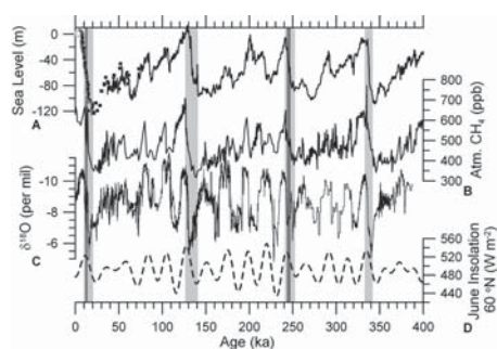
Figure 2. A: Sea level (symbols from Clark et al., 2009; line from Rohling et al., 2009). B: Atmospheric methane ( \text{CH}_4 ) (Petit et al., 1999). C: Chinese speleothem \delta^{18}\text{O} records of East Asian Monsoon (Cheng et al., 2009, and references therein). D: Boreal summer insolation (Berger and Loutre, 1991). Light gray bars denote deglaciations (terminations), while the two dark gray bars denote the Younger Dryas and the Younger Dryas-like event during termination III (i.e., decreased atmospheric methane and East Asian Monsoon (higher \delta^{18}\text{O} )).
