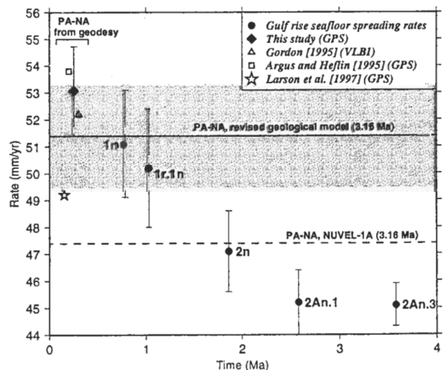
Figure 3. Seafloor spreading rates across the southern spreading segment in the Gulf of California compared to rates predicted at that location by alternative models for PA-NA motion (modified from DeMets [1995]). All uncertainties, including the stippled region, are 1\sigma .
